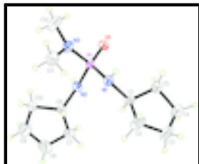
Fig. 1. The molecular structure of the title compound with ellipsoids shown at the 50% probability level.
