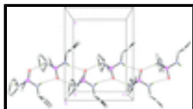
Fig. 2. A view of the crystal packing showing the formation of 1-D arrangement through N—H...O hydrogen bonds (shown as dashed lines). Carbon bound H atoms have been omitted for clarity.
